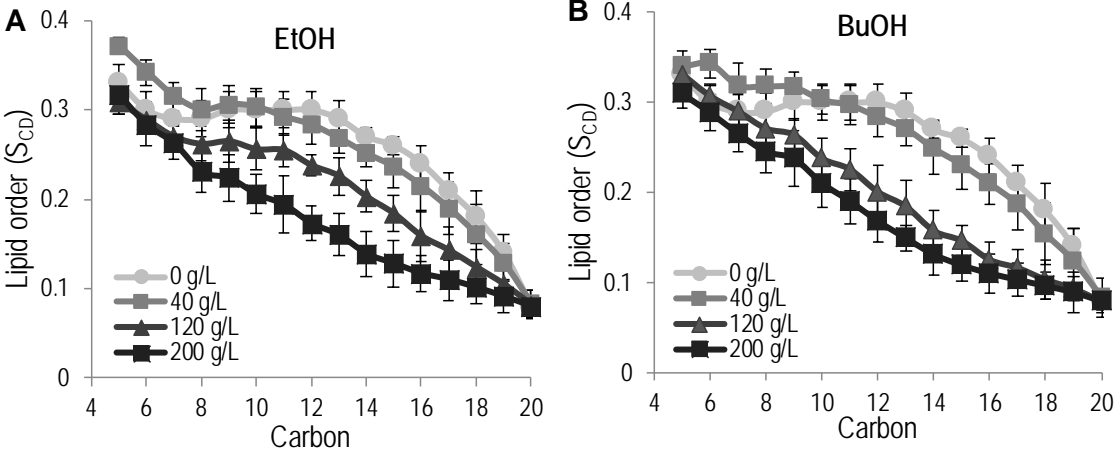
Figure S1: The effect of ethanol and n-butanol on the lipid order of the short chain of IPC. A. Ethanol. B. n-butanol. The data shown are the mean over one simulation \pm standard deviation.
